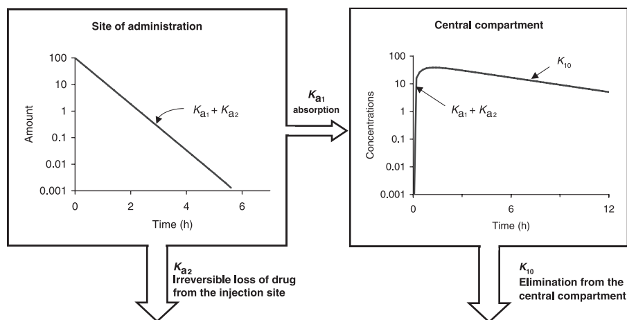
Fig. 12. The so-called half-life of absorption vs. the process of drug absorption. This figure corresponds to a drug obeying a mono-compartmental model with a phase of absorption. The reported half-life of absorption ( t_{1/2} K_a ) does not reflect solely the process of drug absorption (here represented by K_{a1} , the first-order rate constant of drug transfer from the injection site to the central compartment) but the sum of K_{a1} and K_{a2} , K_{a2} being the rate constant reflecting the irreversible loss of drug at the administration site. t_{1/2} K_a reflects simply drug absorption only if K_{a2} = 0 , i.e. if the bioavailability is total. Here K_{a1} + K_{a2} \gg K_{10} and so no flip-flop phenomenon is observed.
